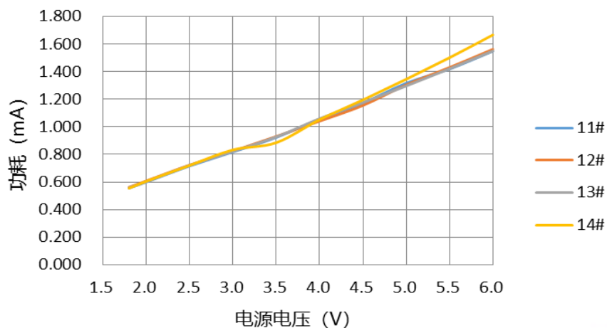
IDD功耗VS电源电压@FCPU=2M@HIRC=32Mhz
