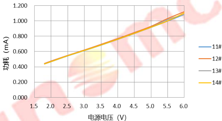
IDD功耗VS电源电压@FCPU=1M@HIRC=32M
