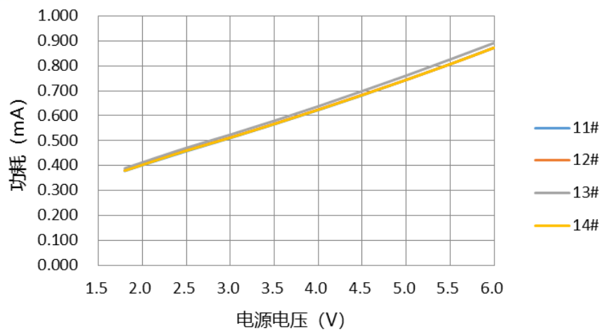
IDD功耗VS电源电压@FCPU=500K@HIRC=32M
